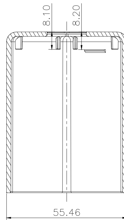
Section E-E
